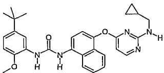
1-(5-tert-Butyl-2-methoxy-phenyl)-3-{4-[2-(cyclopropylmethyl-amino)-pyrimidin-4-yloxy]-naphthalen-1-yl}-urea;
